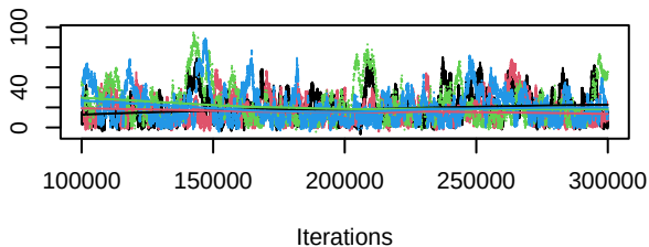
Trace of d.Osimertinib.Osimertinib_chemo
