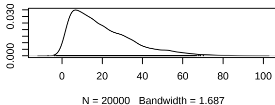
Density of d.Osimertinib.Osimertinib_chemo
