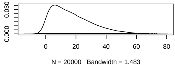
Density of d.Erlotinib.Erlotinib_MMPi
