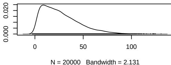
Density of d.Erlotinib.antiangi
