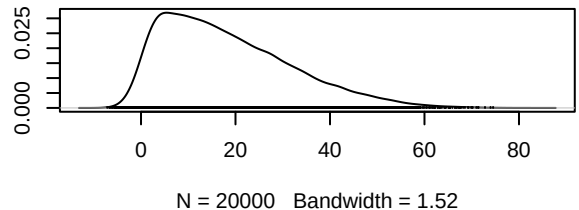
Density of d.Gefitinib.Gefitinib_chemo
